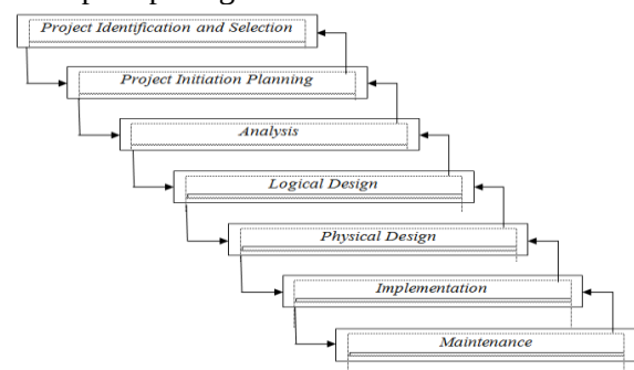
Gambar 2.1 Diagram SDLC
