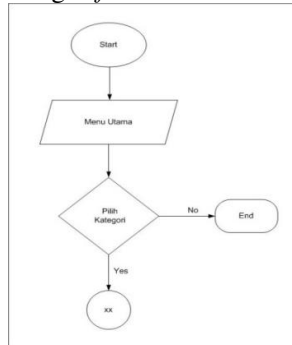
Gambar 1 Flowchart Sistem
